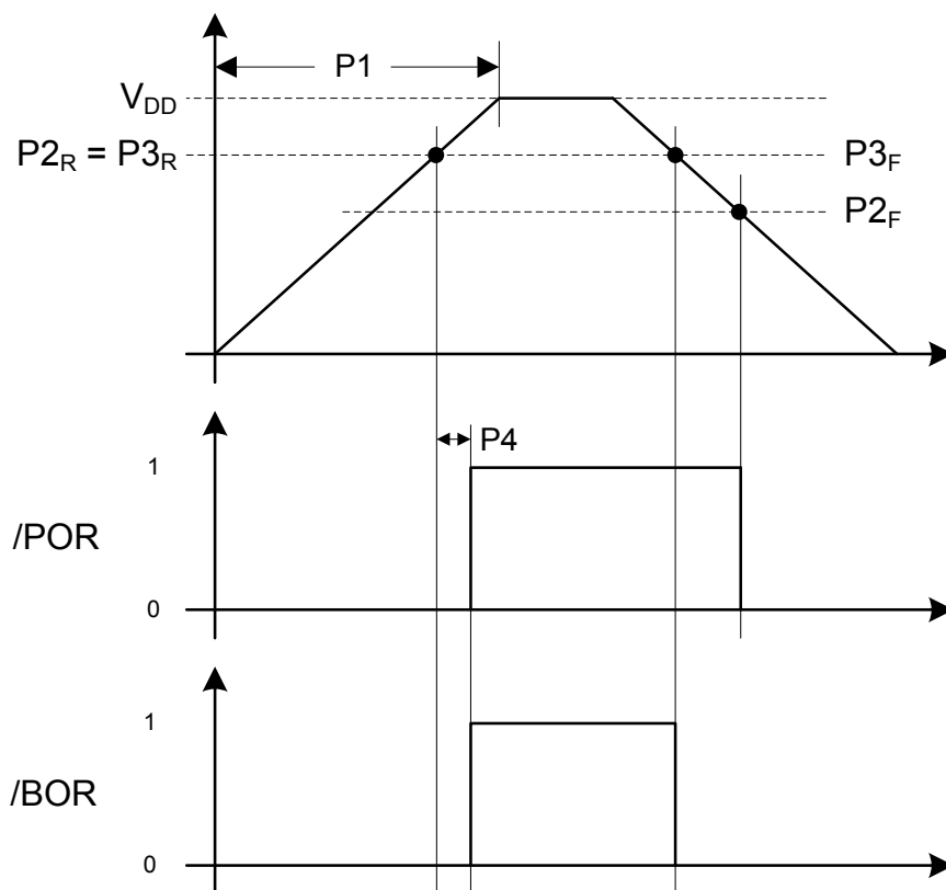
Figure 25-4. Power-On and Brown-Out Reset and Voltage Parameters
