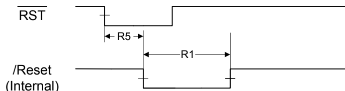
Figure 25-6. External Reset Timing (RST)
